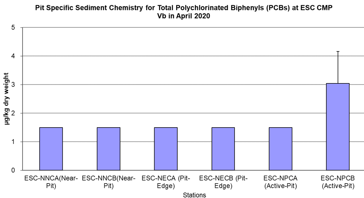
Figure 15: Concentration of Total Polychlorinated Biphenyls (PCBs) ( \mu\text{g}/\text{kg} dry weight; mean +SD) in sediment samples collected from Pit Specific Sediment Chemistry Monitoring for ESC CMP Vb in April 2020.
