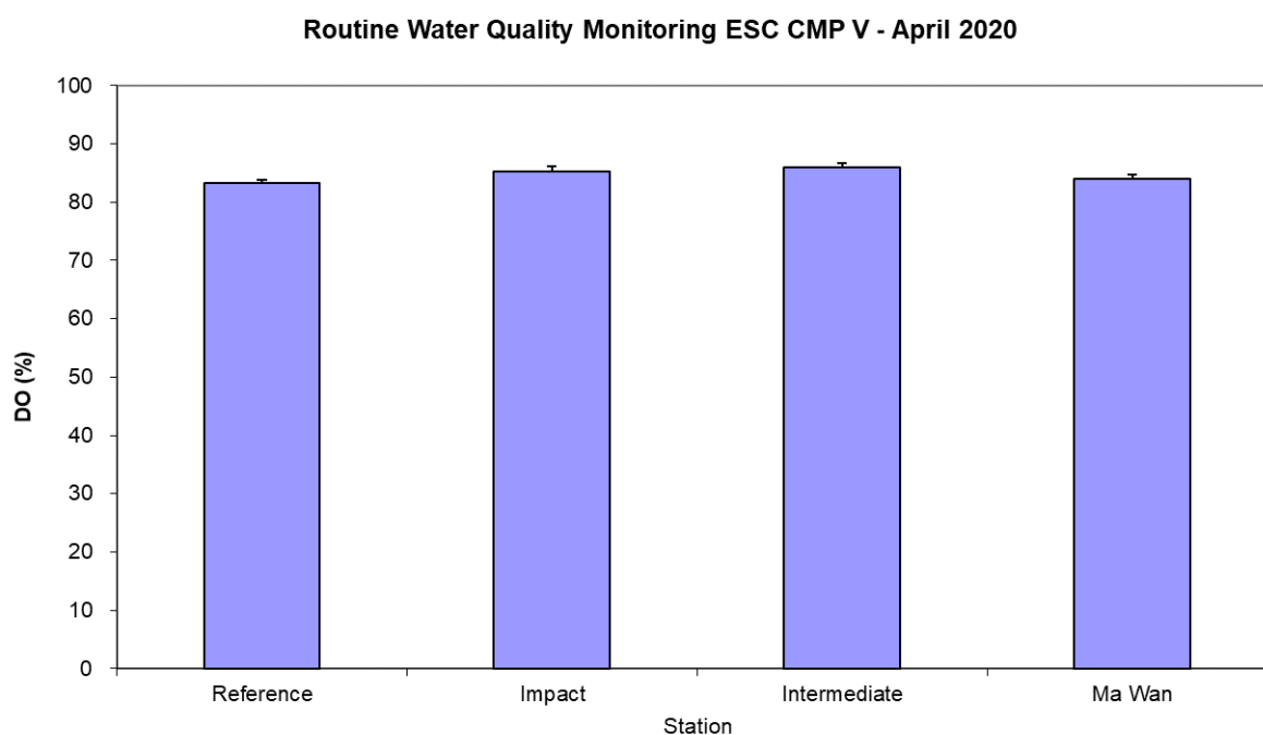
Figure 2: Level of Dissolved Oxygen (DO) (% saturation; mean + SD) recorded during Routine Water Quality Monitoring for disposal operations at ESC CMP V in April 2020.
