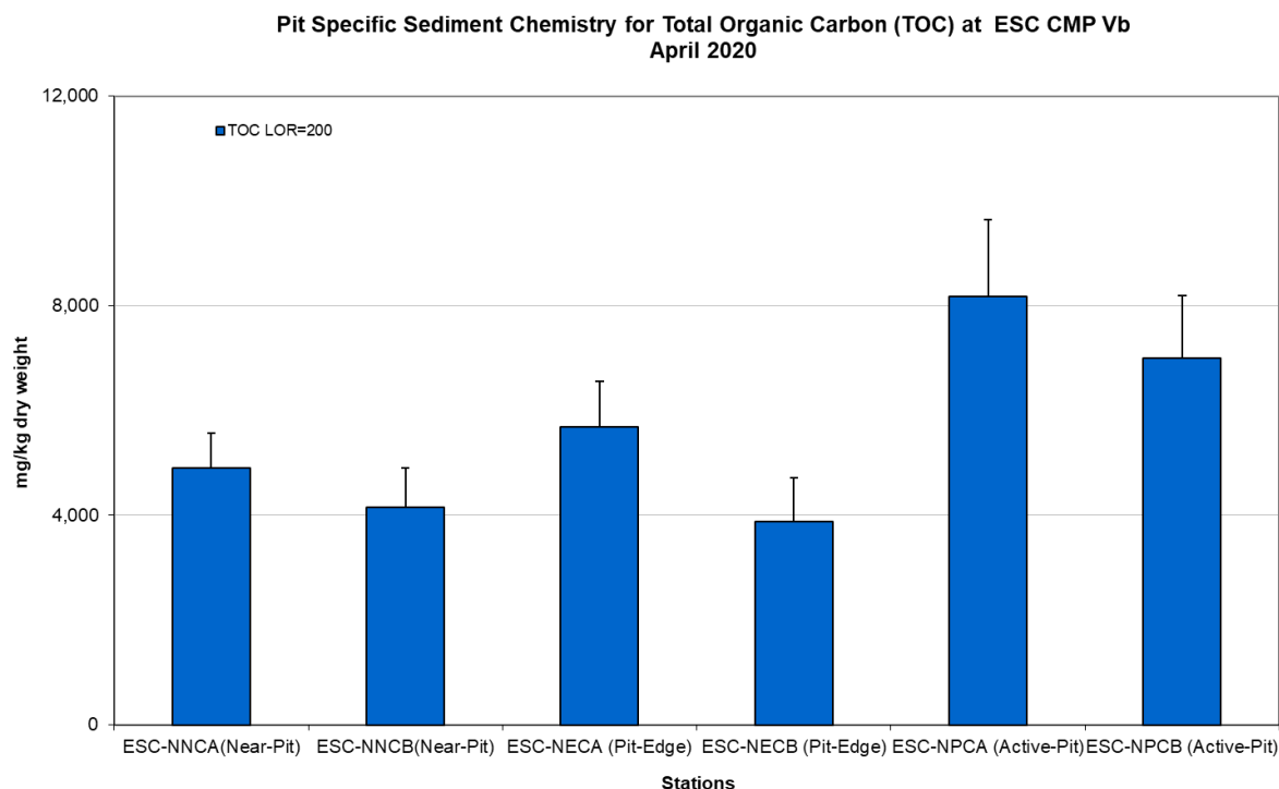
Figure 13: Concentration of Total Organic Carbon (TOC) (mg/kg dry weight; mean +SD) in sediment samples collected from Pit Specific Sediment Chemistry Monitoring for ESC CMP Vb in April 2020.
