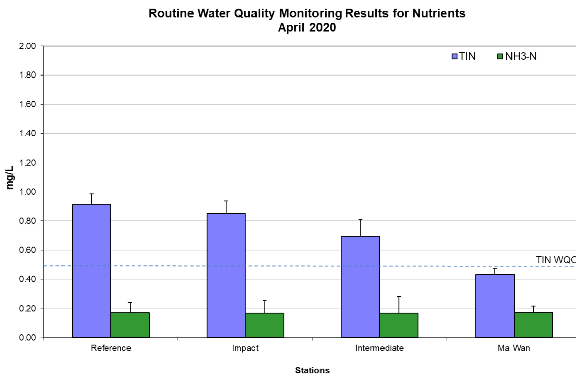
Figure 8: Concentration of Total Inorganic Nitrogen (TIN) and Ammonia Nitrogen ( \text{NH}_3\text{-N} ) ( \text{mg/L} ; mean + SD) in water samples collected from Routine Water Quality Monitoring for disposal operations at ESC CMP V in April 2020.
