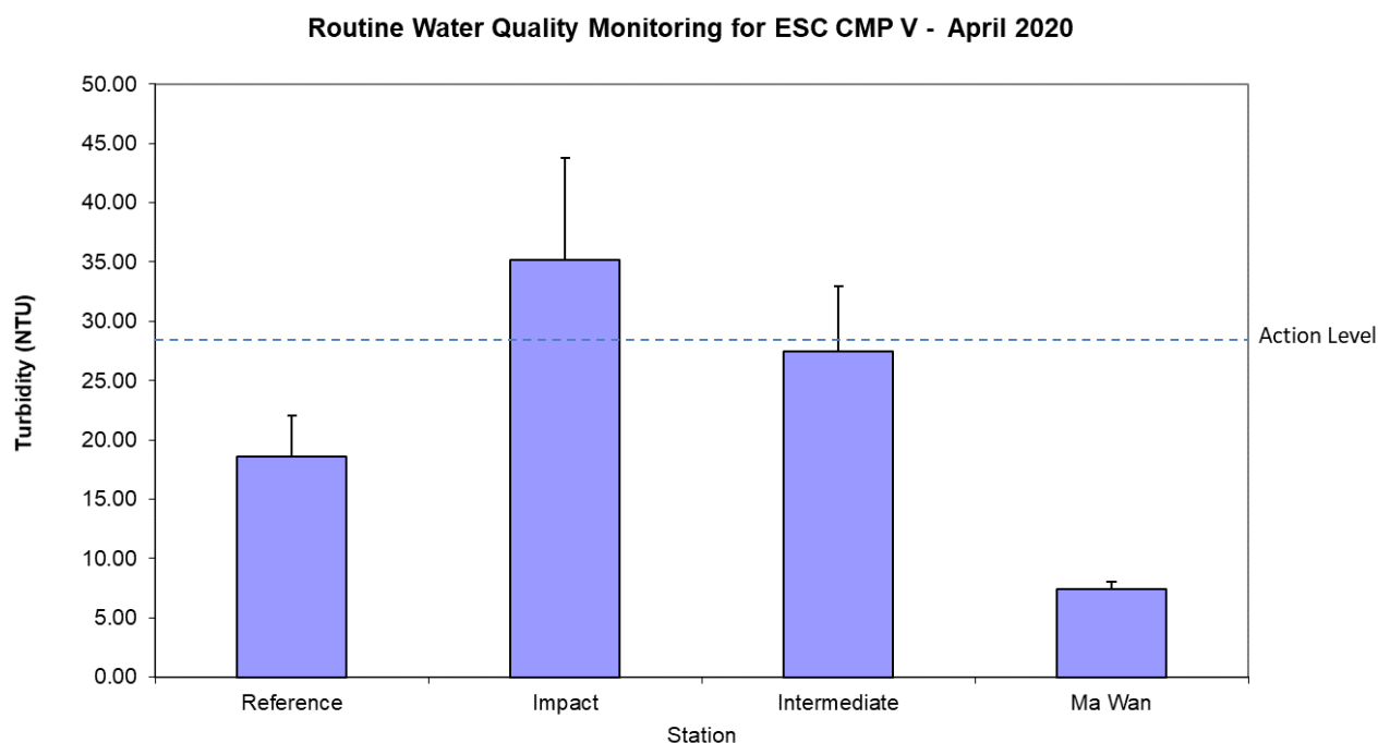
Figure 6: Levels of Turbidity (NTU; mean + SD) recorded during Routine Water Quality Monitoring for disposal operations at ESC CMP V in April 2020.
