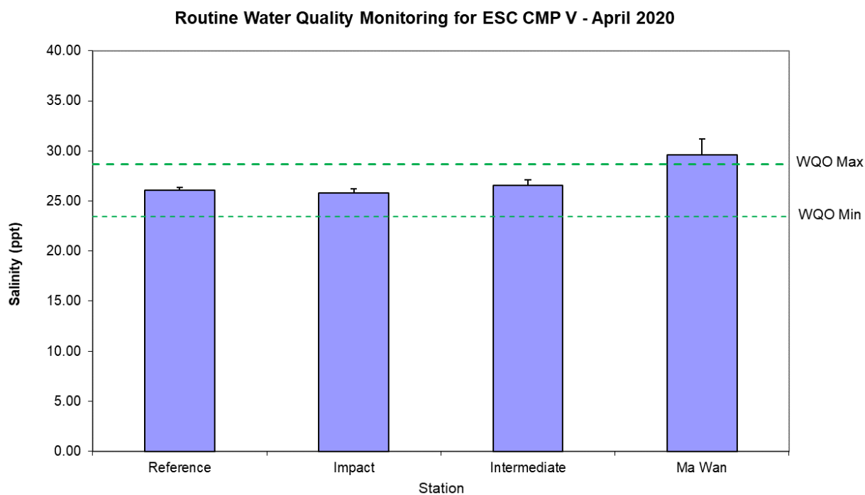
Figure 5: Level of Salinity (ppt; mean + SD) recorded during Routine Water Quality Monitoring for disposal operations at ESC CMP V in April 2020.
