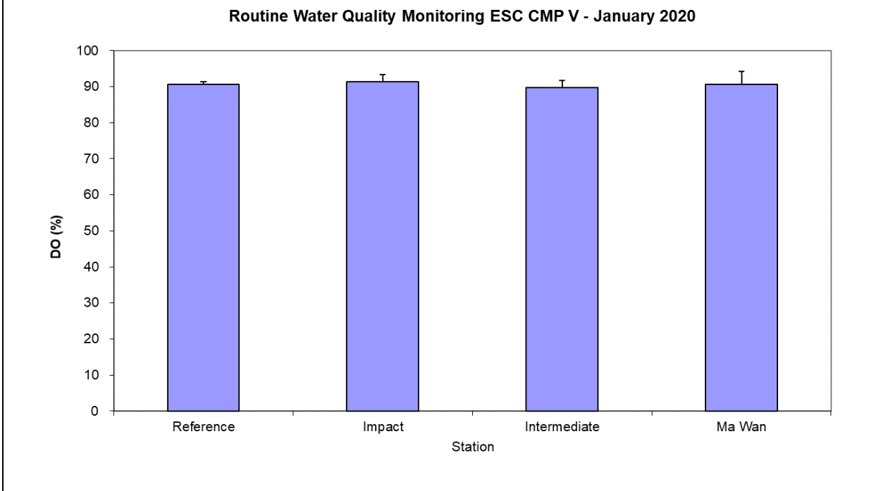
Figure 2: Level of Dissolved Oxygen (DO) (% saturation; mean + SD) recorded during Routine Water Quality Monitoring for disposal operations at ESC CMP V in January 2020.
